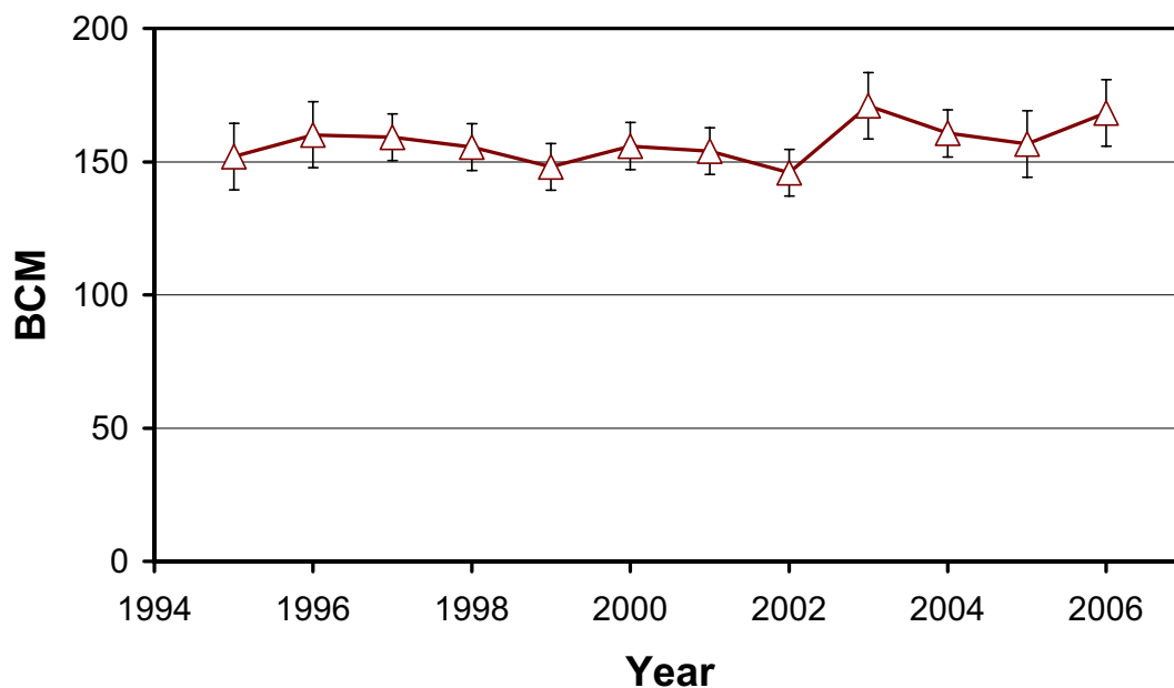
Figure 14. Global gas flaring has remained largely stable for the past fifteen years.
