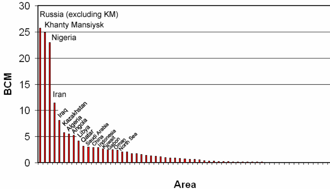
Figure 13. Year 2004 gas flaring estimates in billions of cubic meters (BCM).
