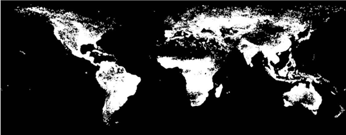
Figure 19. Plot of all the MODIS active fire detections from 2004.
